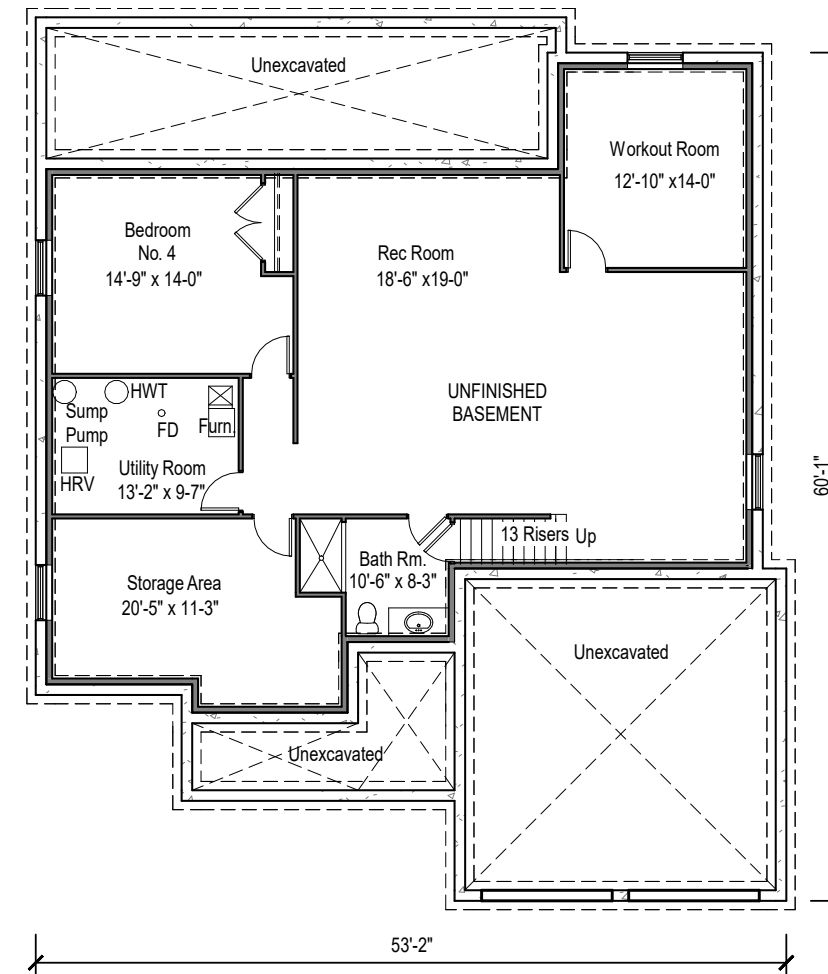
Optional Basement Floor Plan
