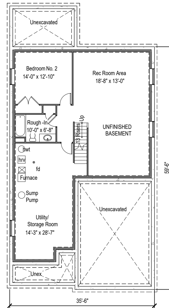
Optional Basement Floor Plan
