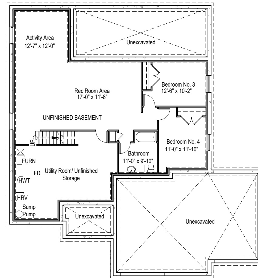
Optional Basement Floor Plan
