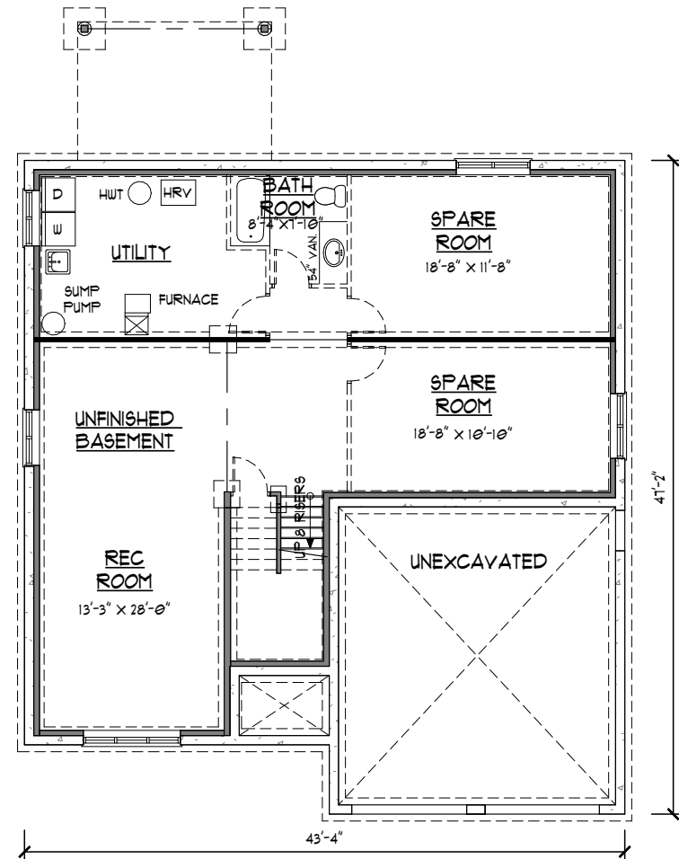
OPTIONAL BASEMENT FLOOR PLAN
